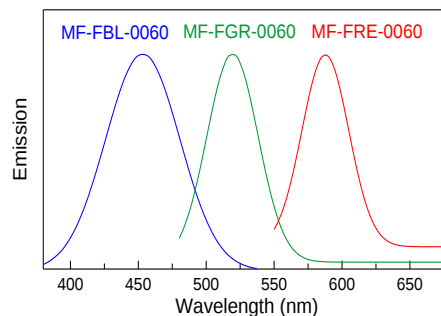
Fig1. Emission spectra of FluoroNanoQ.
